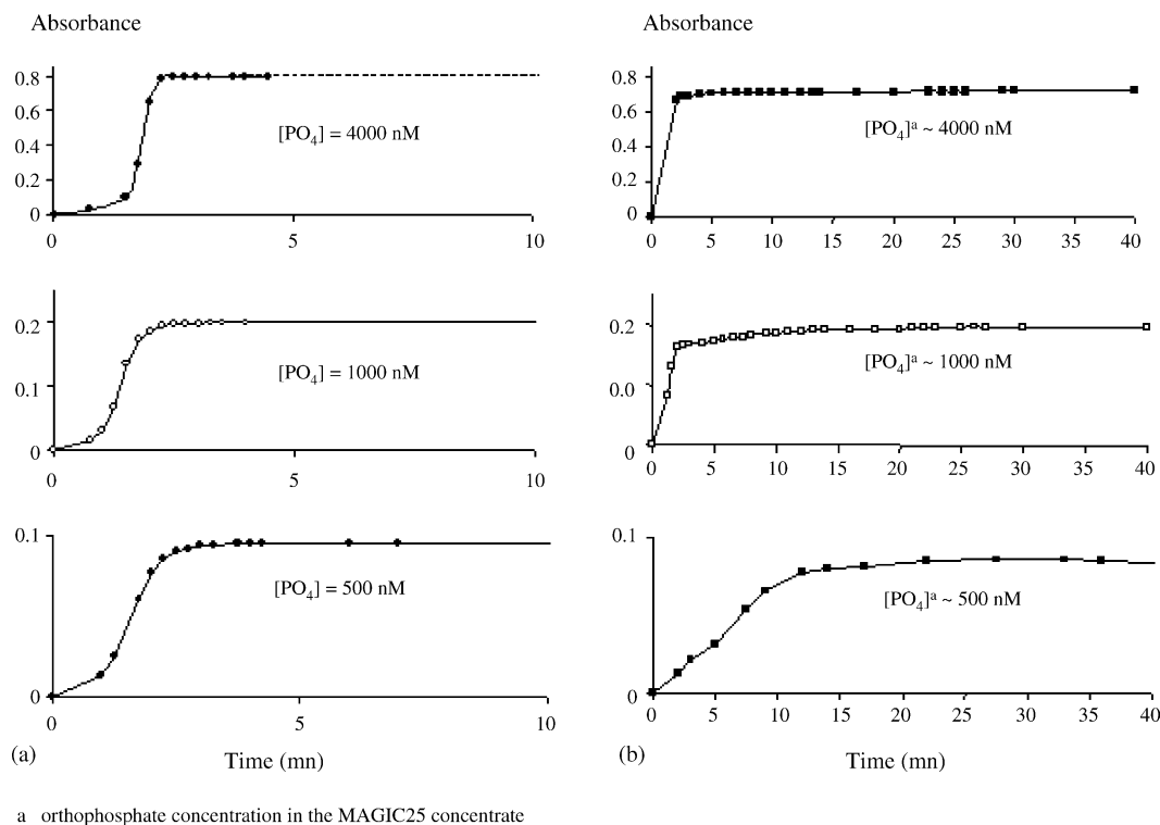
Fig. 2. Absorbance vs. time: reaction rate curves of orthophosphate solutions in seawater (a) and in MAGIC25 concentrate (b).
