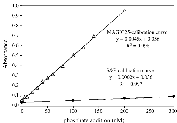
Fig. 1. Typical calibration curves of S&P and MAGIC25 method.
