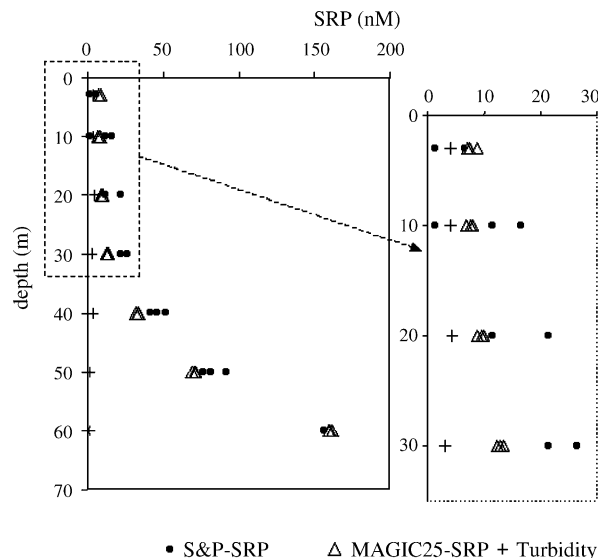
Fig. 6. SRP profiles with MAGIC25- and S&P-methodology, at DYFAMED station (43°25'N, 7°52'E), April 2004.
