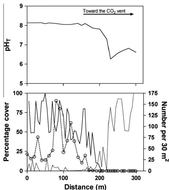
Fig. 7. (Top) Variation of pH along a transect toward a \text{CO}_2 vent south of Castello d'Aragonese (Ischia, Italy). (Bottom) Along the same transect, the abundances of key species of this ecosystem. The percentage cover (left axis) of calcareous (solid line) and non-calcareous algae (dotted line) as well as the abundance (right axis) of sea urchins (dotted line, open circles) are shown. Data are from Hall-Spencer et al. (2008).
