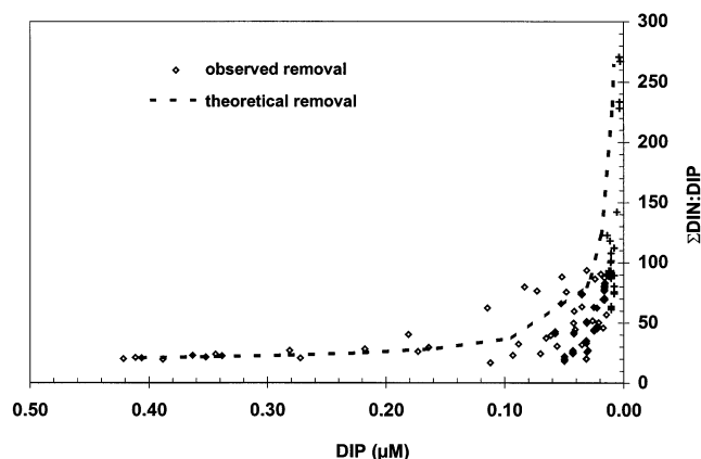
Fig. 6. \text{NO}_3^- :DIP versus DIP relationship. ( \diamond ) Data; (+) ratios obtained from DIP data below the detection limit. Dashed line represents the theoretical curve of phytoplankton DIP utilization with corresponding \text{NO}_3^- :DIP ratios in upwelled deep Mediterranean water ( \text{DIN:DIP} = 22 , and \text{DIP} = 0.41 \mu\text{M} ). The typical Redfield (1958) ratio of N:P requirements (16:1) for phytoplankton was used in the model
