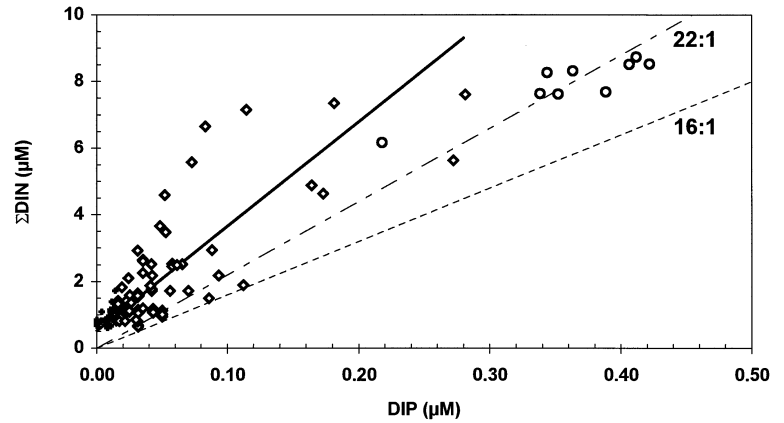
Fig. 3. \Sigma\text{DIN} versus DIP relationship. (◇) From 0 to 150 m layer; (+) points based on the DIP data below the detection limit; (○) from the 200 to 400 m layer. Solid line represents the linear regression (model II, Sokal & Rohlf 1995: \Sigma\text{DIN} = 31.34\ \text{DIP} + 0.53 , r^2 = 0.647 , n = 136 ) of data from the 0 to 150 m layer. Dashed and dashed-dotted lines indicate the 16:1 (global ocean) and 22:1 (Mediterranean waters) ratios, respectively
