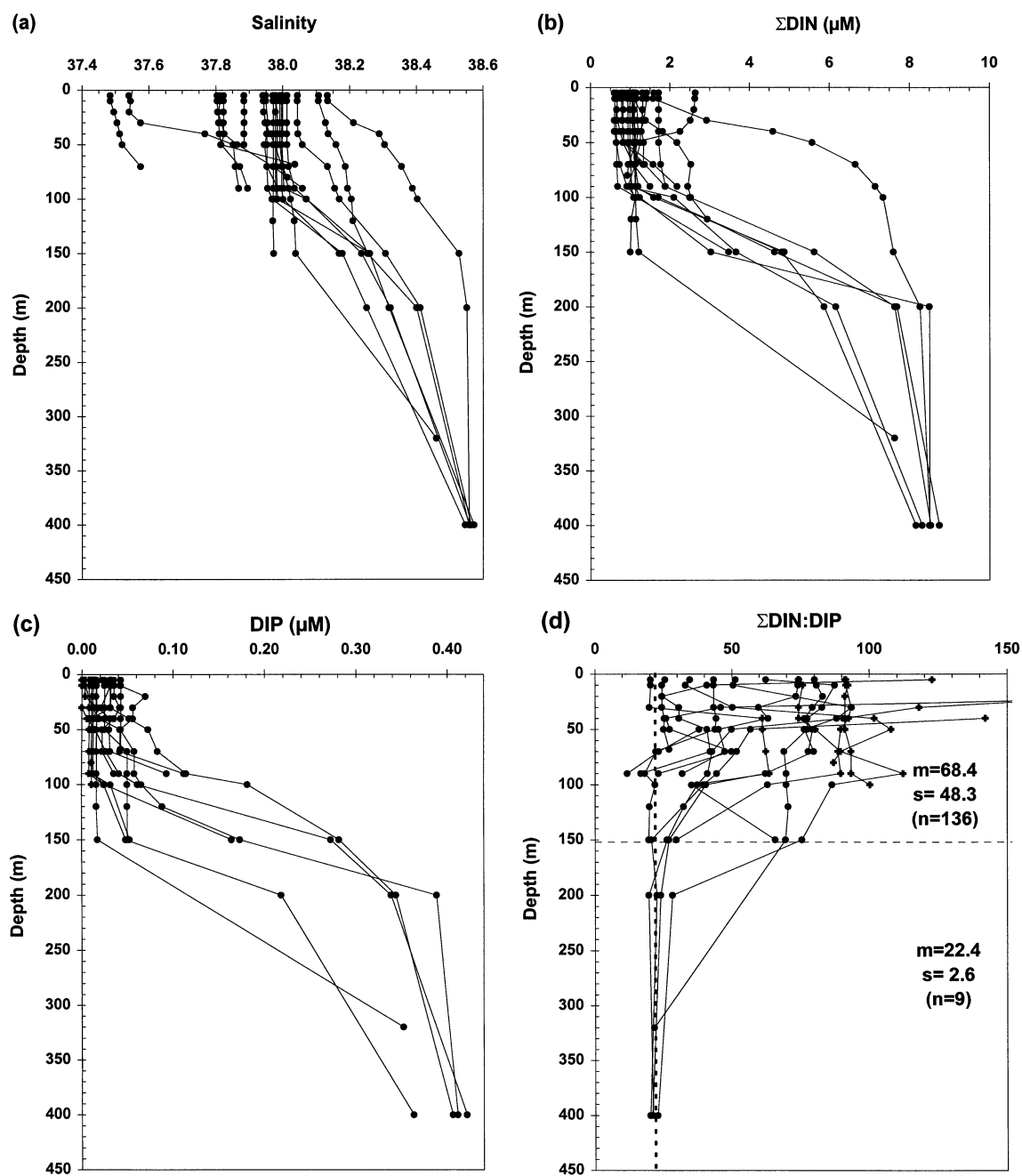
Fig. 2. (a) Salinity, (b) \Sigma\text{DIN} ( \text{NO}_3^- + \text{NO}_2^- + \text{NH}_4^+ ), (c) phosphate (DIP) and (d) \Sigma\text{DIN:DIP} molar ratio versus depth at the 20 stations of the MOOGLI 1 Cruise. The vertical dashed line in (d) indicates the value of the \text{NO}_3^-:\text{DIP} ratio (=22) reported by McGill (1969) for the Mediterranean area. Mean ( m ), standard deviation ( s ) and the number of data ( n ) of \text{NO}_3^-:\text{DIP} ratios were computed for 2 distinct layers (0 to 150 and >150 m). (+) Data representing or based on DIP concentrations below the detection limit
